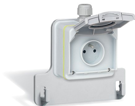
Prise renforcée Green'up Access et patène de suspension
